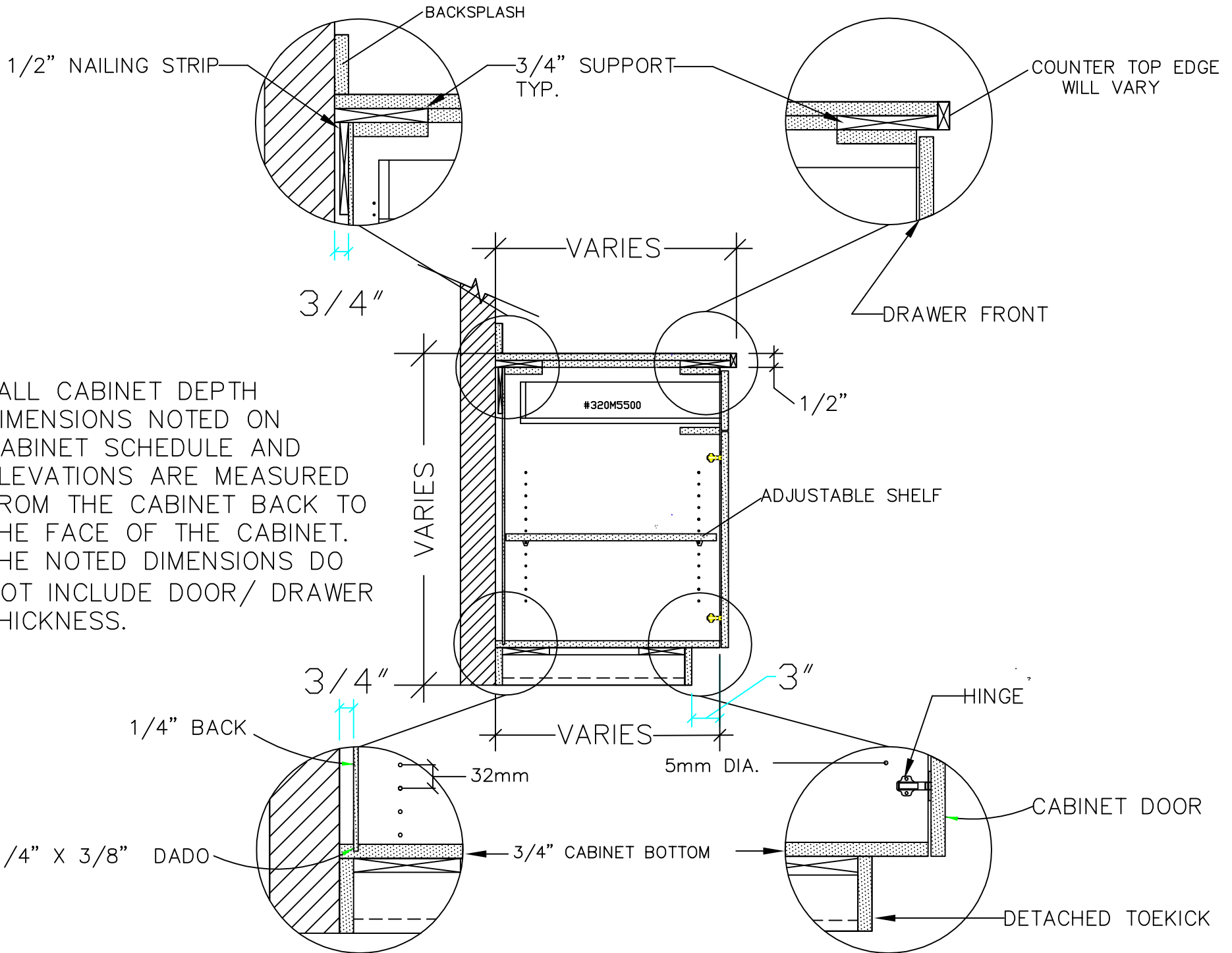
DETAIL D-6
